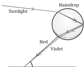
Figure 11.8 Rainbow formation
