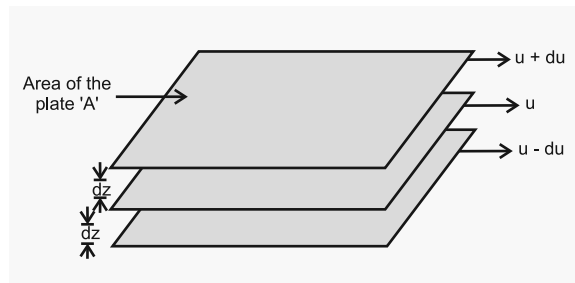
Fig. 5.14 Gradation of velocity in the laminar flow
