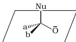
Fig.12.2: Nucleophilic attack on carbonyl carbon
